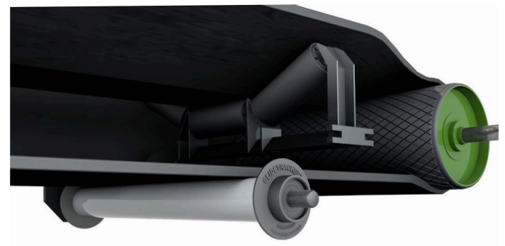
Glidetracker™ fitted at tail section to improve feed point tracking
